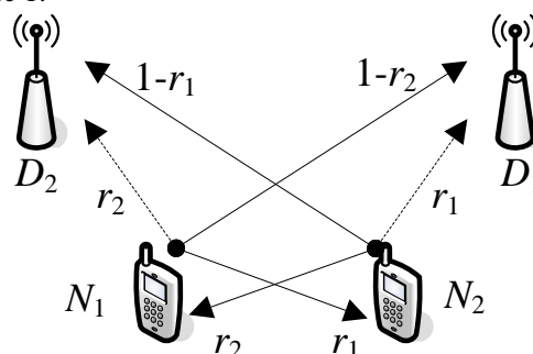
FIGURE 1 The system model for cooperative transmission
