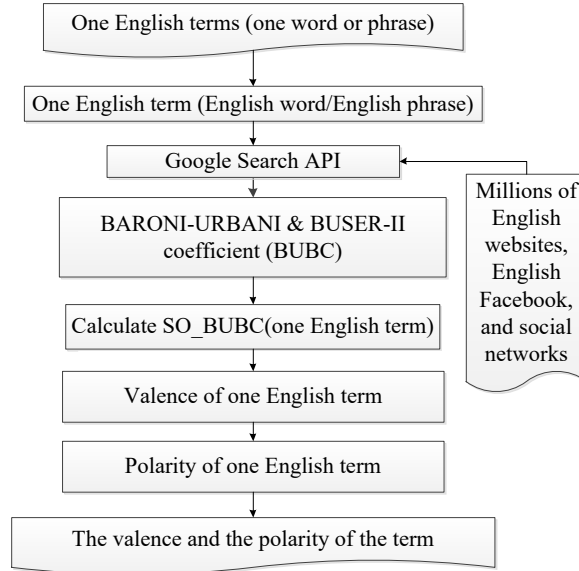
FIGURE 3 Overview of identifying the valence and the polarity of one term in English using a BARONI-URBANI & BUSER-II coefficient (BUBC)
