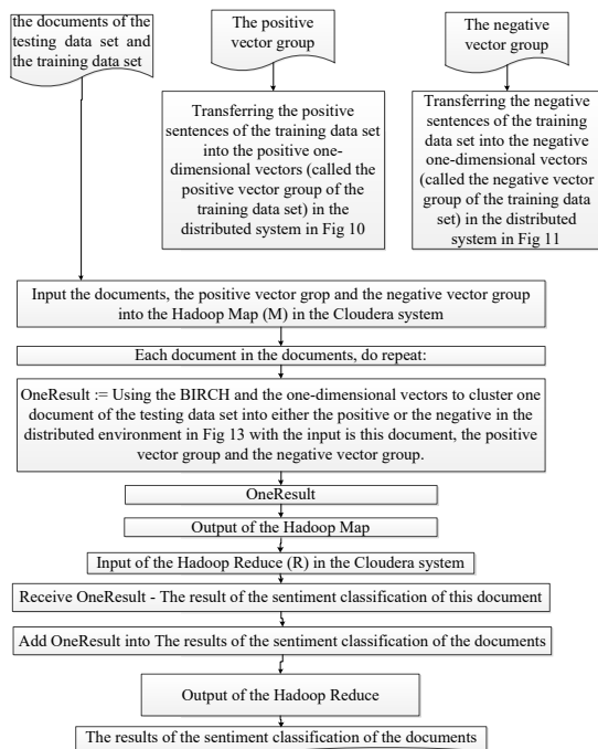
FIGURE 14 Overview of using the BIRCH and the one-dimensional vectors to cluster the documents of the testing data set into either the positive or the negative in the parallel network environment.
